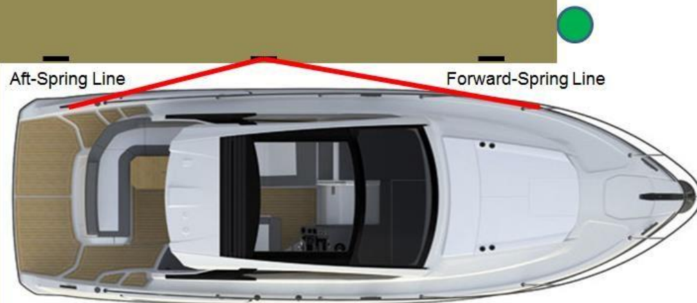
Figure 8 – Spring lines run to middle of finger
