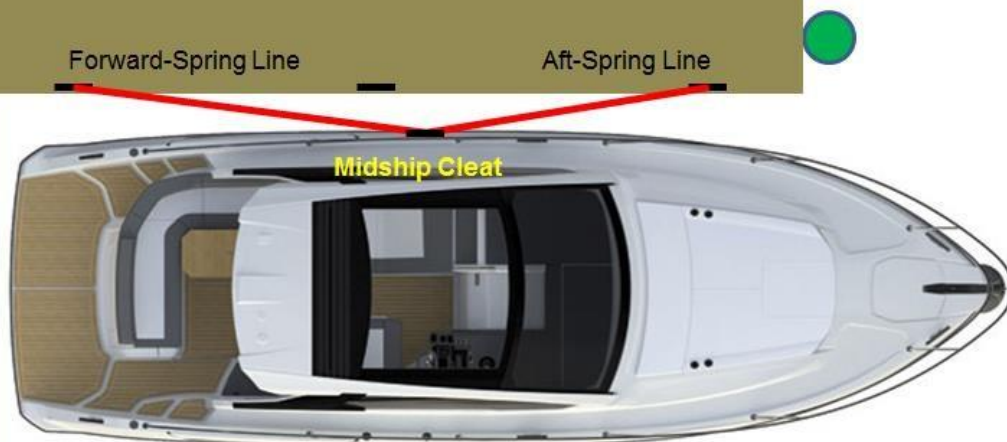
Figure 9 – Spring lines run from finger to boat's midship cleat
